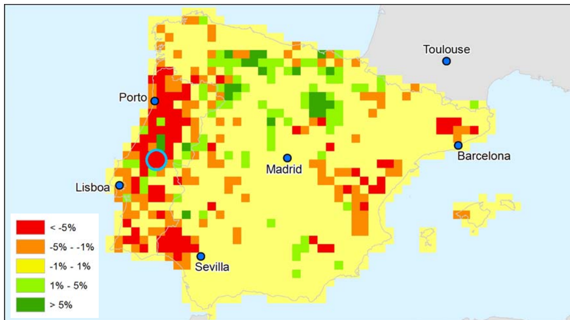
Figure 7. Trend in forest connectivity in the Iberian Peninsula, 1990-2006 (insight where blue circle in figure 8)
