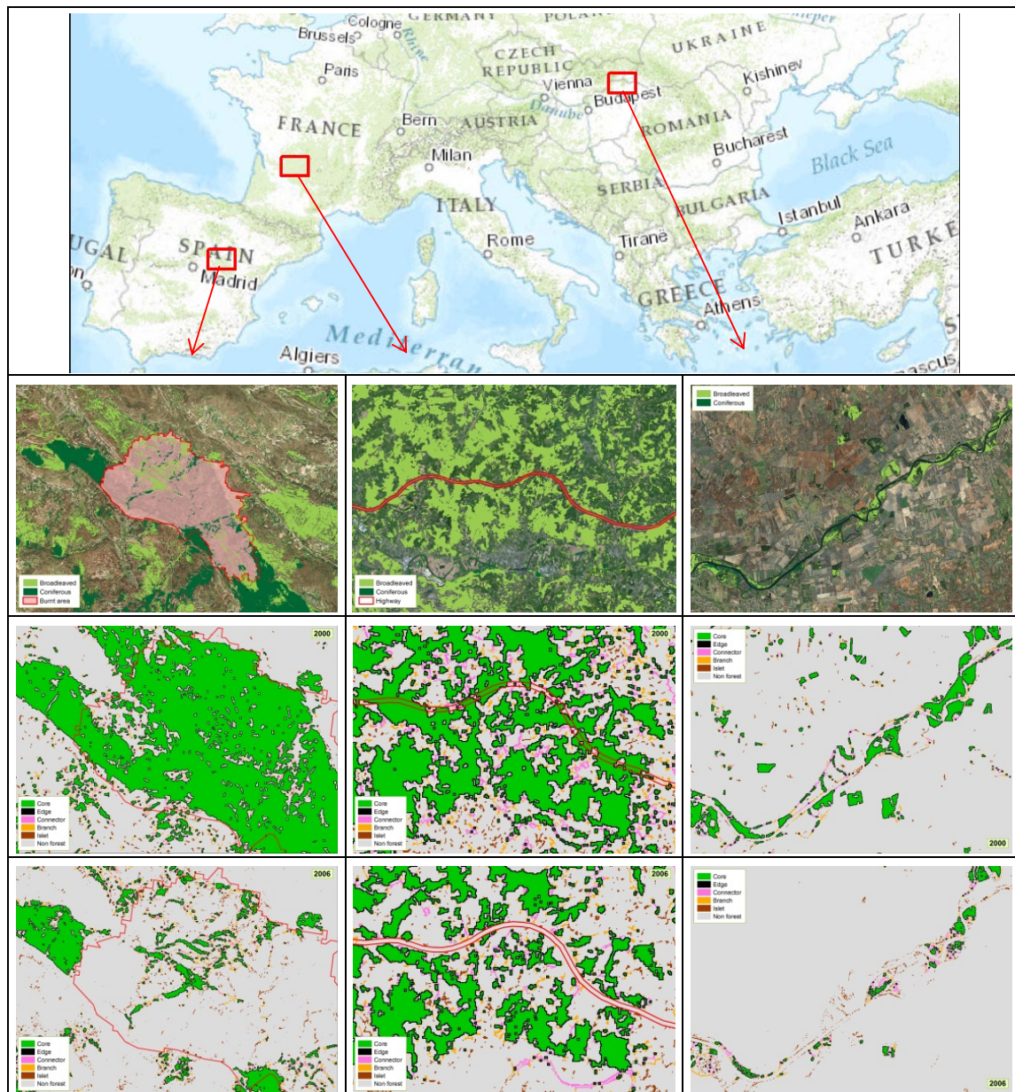
Figure 1. Fragmentation examples due to, from left to right, a fire, a trans-European highway and forest clearance along a riparian area (data: JRC forest maps 2000 and 2006)
